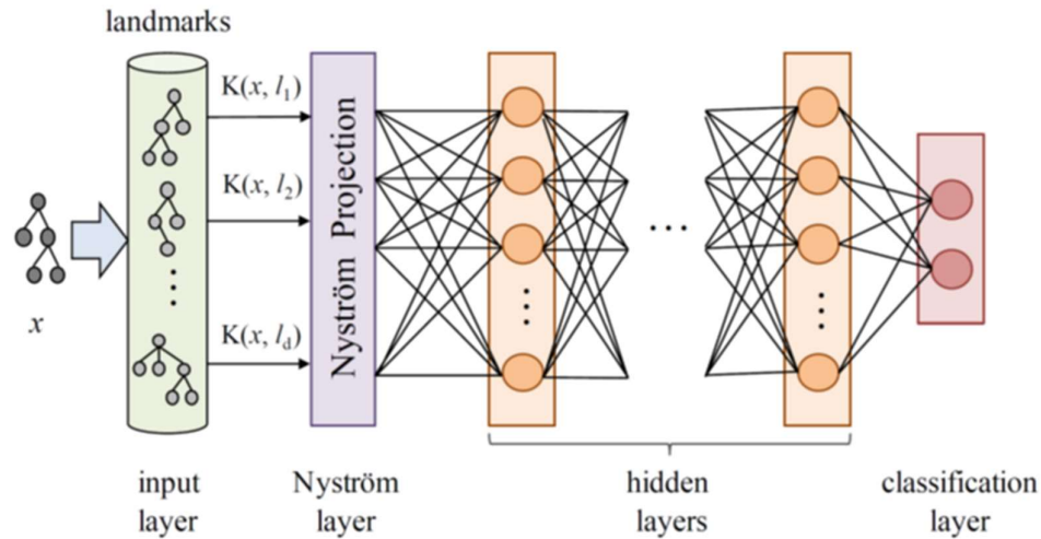
Figure 1 - Kernel-based Deep Architecture
