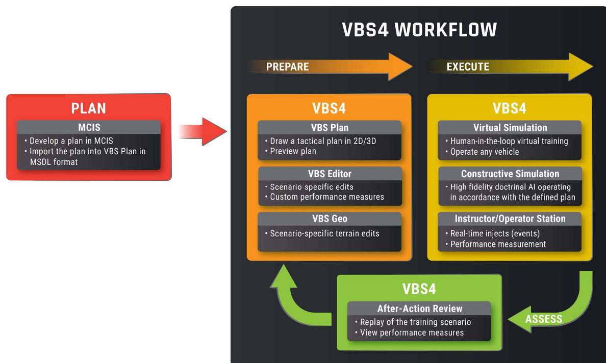
Figure 2 – The VBS4 workflow
